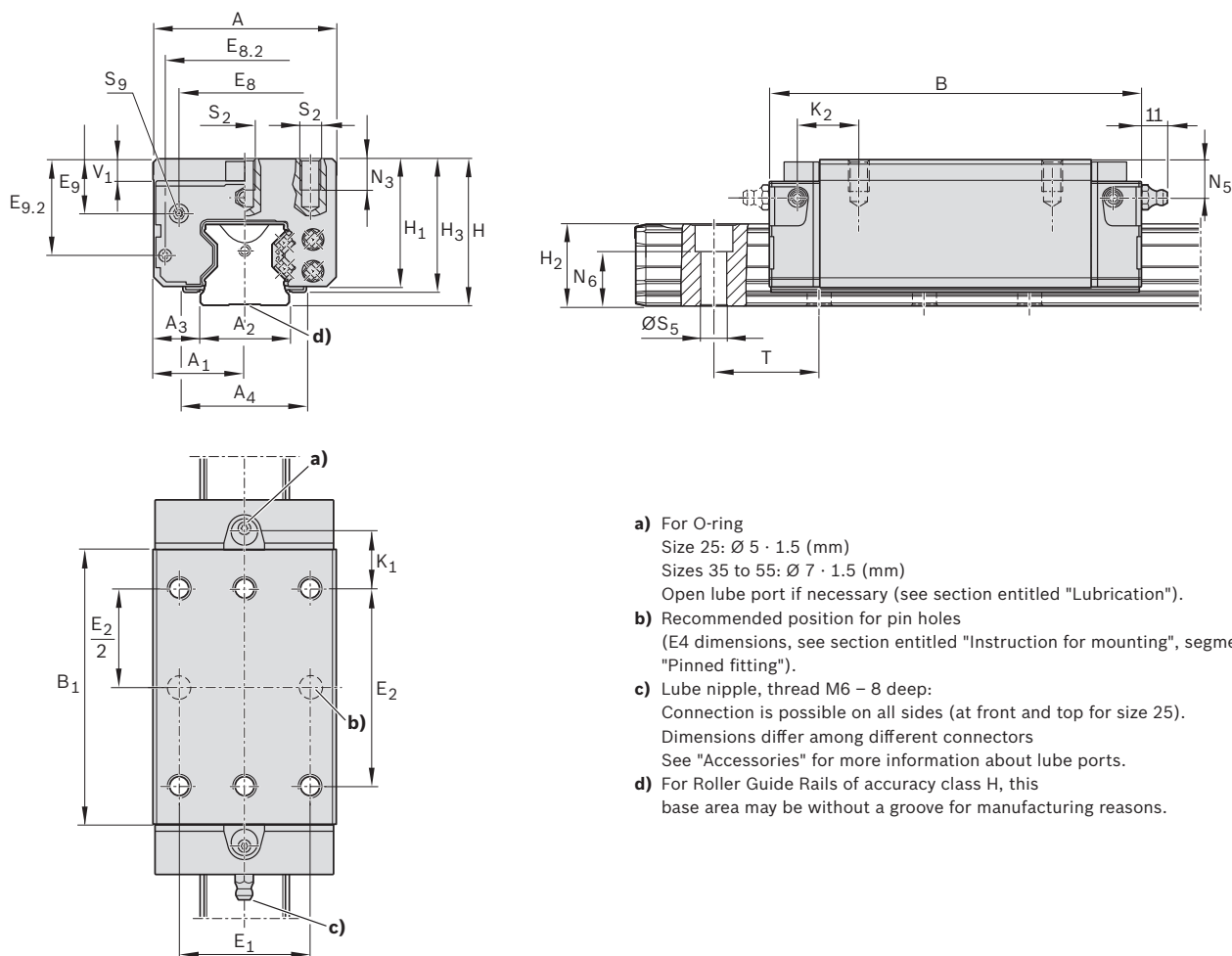
Dimensions (mm)
