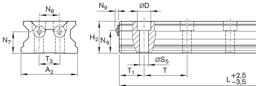
Roller Guide Rail with cover strip and threaded holes on end faces. Retaining with screws and washers (included).
