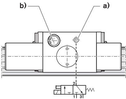
Circuit for standard air port
