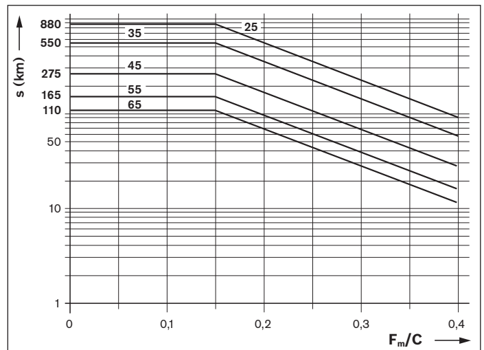
Fig. 1 Relubrication interval
