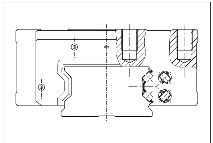
Optimum design of the Roller Guide Rail
