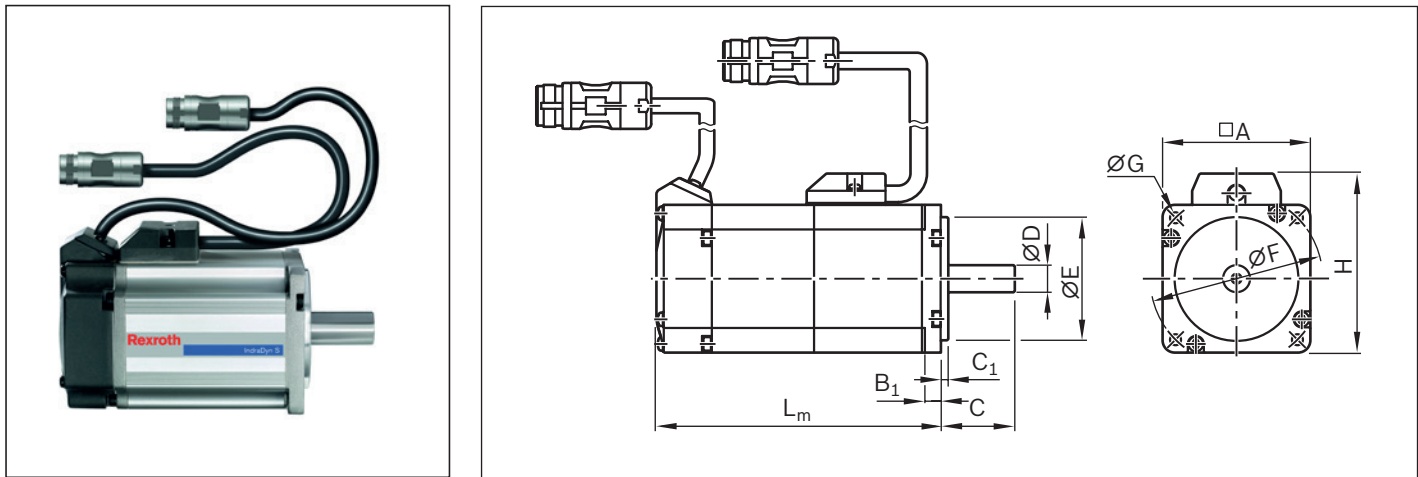
Motor schematic
